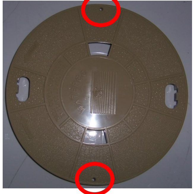
Two retaining screw holes moulded into the Skimmer Box lid to secure to retaining insert ring.
