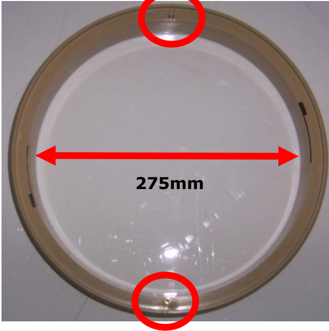
Two retaining screw inserts moulded in the Skimmer Box retaining insert ring.
